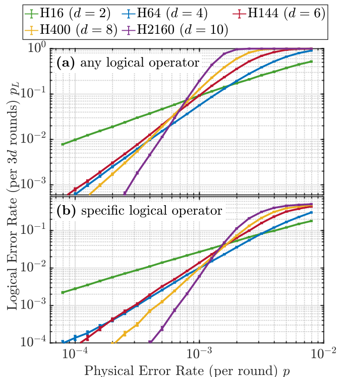
Figure 6. Logical error rates for the family of hyperbolic Floquet codes listed in Table I. (a) The any logical operator error rate. An error in any of the 2k logical operators of each code is considered a logical error for this rate. (b) The specific logical operator error rate. For this rate, failure or success of the decoder is defined based on having an error or not impacting a specific logical operator within 2k logical operators of each code. Since hyperbolic Floquet codes are based on symmetric graphs, the choice of the specific logical operator does not matter for obtaining this plot.
