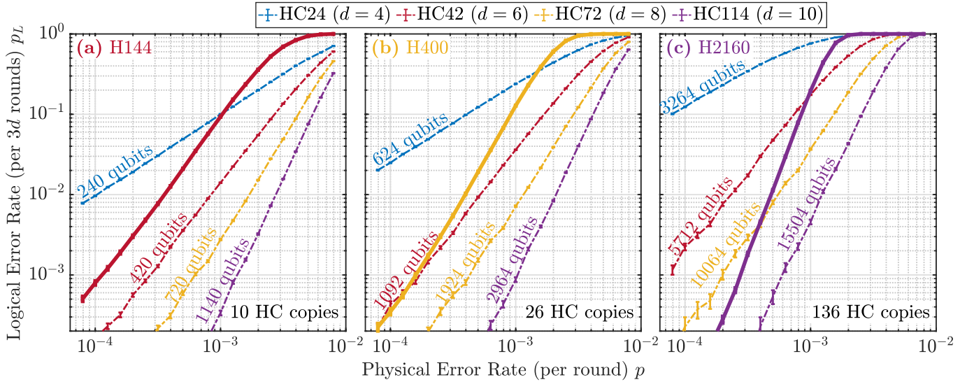
Figure 7. Comparison between hyperbolic and honeycomb Floquet codes. Panels (a), (b), and (c) show the any logical operator error rate of H144, H400, and H2160 hyperbolic codes (solid lines) compared to 10 copies, 26 copies, and 136 copies of honeycomb codes (dashed lines), respectively. Honeycomb codes are denoted by HC followed by their number of physical qubits. Each honeycomb code stores two physical qubits. The number of copies of honeycomb codes is chosen such that the total number of logical qubits in each panel equals to k of the respective hyperbolic code. The total number of physical qubits needed for that many copies of honeycomb codes is noted alongside the respective dashed line.
