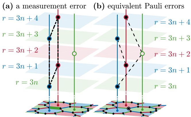
Figure 5. Detection events of a measurement error. (a) The faulty measurement outcome of the highlighted green check at round r = 3n is used to infer an incorrect value for the adjacent blue and red plaquette syndromes at rounds r = 3n and r = 3n + 1 . Later correct measurement of the same check leads to correct inference of these syndromes three rounds later. In both cases, the inferred syndrome differs from the most recent inference and gives rise to a detection event. Hence, a measurement error has four detection events forming a hyper-edge in the syndrome lattice, shown with a dashed parallelogram. (b) A combination of three simple Pauli errors on one of the qubits of the faulty check, denoted with a circle, gives rise to the same detection events. These equivalent Pauli errors have the same effects on the logical operators as the measurement error.
