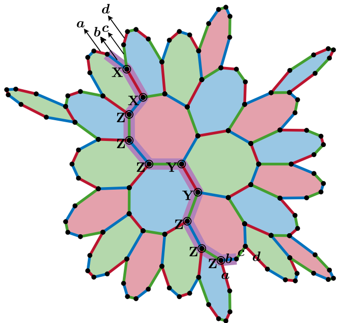
Figure 1. A hyperbolic Floquet code with 64 physical qubits. The code is based on an octagonal \{8, 3\} lattice, which is displayed using polar coordinates of its vertices. The 64 physical qubits are located at the vertices of the lattice. Identification of the edges at the boundary makes the lattice a periodic tessellation of a genus-5 manifold. Four such periodic boundary condition identifications are marked by letters a-d . The octagonal faces are three-colored such that the adjacent faces have different colors. Each edge inherits the color from the two faces it would enter if elongated. Green, blue, and red edges correspond to XX , YY , and ZZ measurement checks, respectively. The blue edges at the ends of the highlighted purple path are identified as a periodic boundary condition, marked with letter b . The purple path therefore is a closed path consisting of 10 unique vertices, marked by circles. This closed path hosts a weight-10 noncontractible loop operator, Pauli operators of which are denoted next to its vertices.
