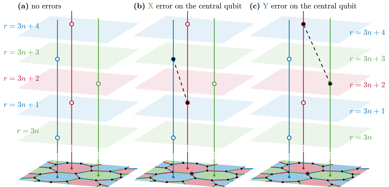
Figure 4. Detection events for Pauli errors. (a) (2+1)D lattice of plaquette syndromes. Each plaquette syndrome is inferred every third measurement round, denoted by empty circles in the timelines of the plaquettes. (b) X and (c) Y Pauli errors between rounds r = 3n and r = 3n + 1 lead to detection events marked on lines perpendicular to the hyperbolic plane. In the presence of errors, inference of a plaquette syndrome may yield a value different than its most recent inferred value. In this case, the inferred syndrome exhibits a detection event, denoted by a filled circle. For the Pauli errors happening between rounds r = 3n and r = 3n + 1 , X and Y Paulis are simple Pauli errors and are associated with two detection events, connected to each other by an error edge in the syndrome lattice. A Z Pauli, on the other hand, is a compound Pauli error and is equivalent to a combination of these X and Y Paulis encompassing all four detection events. The four detection events of a compound Pauli error form a hyper-edge in the syndrome lattice.
