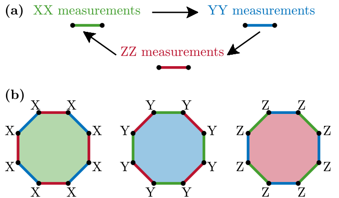
Figure 2. Measurement protocol and plaquette operators of hyperbolic Floquet codes. (a) One cycle of the Floquet code's measurement protocol. Each cycle consists of three measurement rounds, each round carried out on XX, YY, and ZZ checks, corresponding to green, blue, and red edges in Fig. 1, respectively. In each measurement, the weight-two Pauli operator of the two qubits at the ends of that edge are measured. (b) Plaquette operators that are products of checks along the edges of each octagon, for green, blue, and red plaquettes. They commute with all check operators on the lattice, and their value can be inferred using the measurement outcomes of the check operators.
