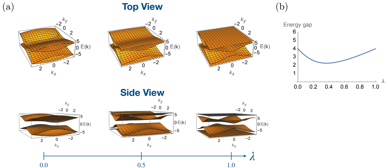
FIG. 11. (a) The Bogoliubov quasiparticle bands of the interpolating Hamiltonian H_{p_x + ip_y, x}(\lambda) in Eq. (11) with t = 1.0 , \mu = -2.0 , \mu' = -8.0 , and \Delta = 1.0 . Along the entire path, the many-body ground state has the lower two (i.e. negative-energy) quasiparticle bands filled and the upper two (i.e. positive-energy) bands empty. Along the entire path, it takes a finite amount of energy to create a quasiparticle in the upper bands or remove a quasiparticle from the lower bands. This demonstrates that the many-body system is gapped throughout the adiabatic evolution for horizontal entanglement renormalization. There is no hopping or pairing for blue B sites at the end of the adiabatic process, so we get two flat bands at \lambda = 1 . (b) We restrict the Hamiltonian to the same fermion parity superselection sector as the ground state and, within this restricted Hilbert space, plot the spectral gap above the many-body ground state.
